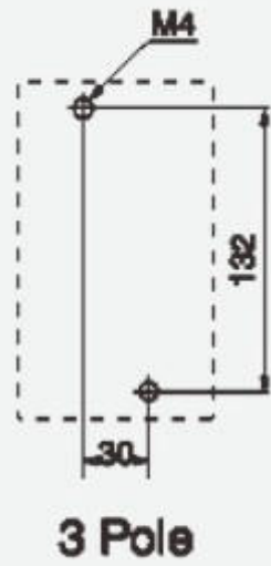
Diagram of terminal connection
